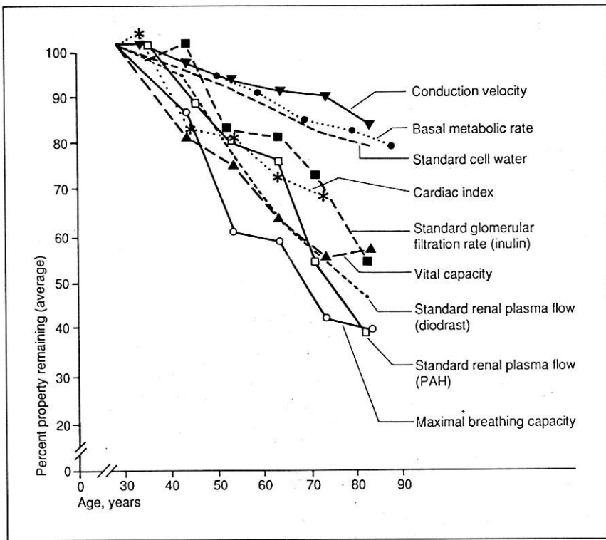
Fig. 2. Age changes in physiologic functions, expressed as a percent of mean value at age 30 years; data are derived from cross-sectional studies [11].
