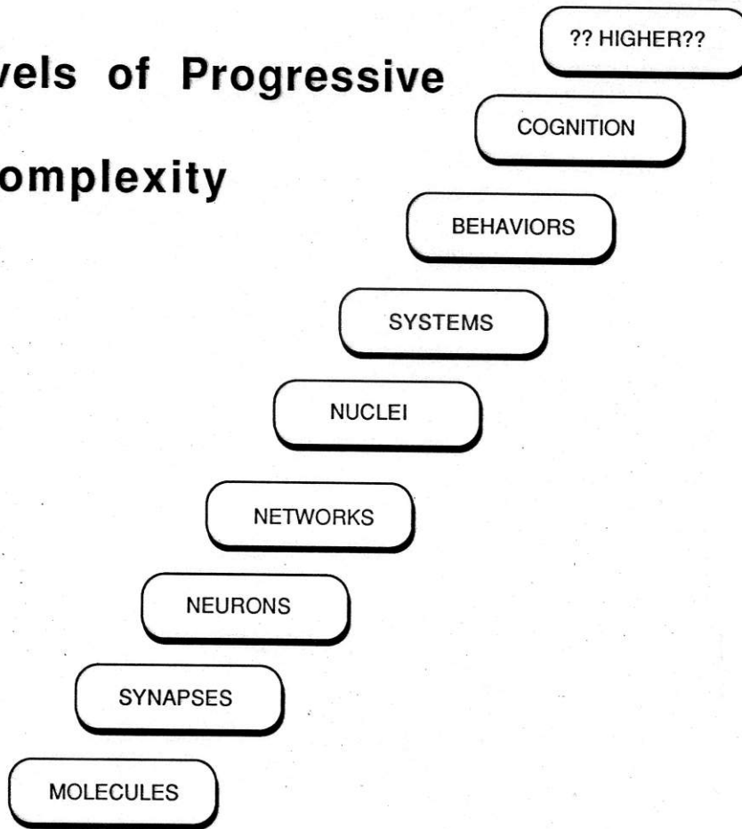
Figure 4. A vertical hierarchical scheme suitable for extending the analysis of a given neurotransmitter molecule from the molecular level of resolution through the circuits in which it is involved with cell ensembles and systems to regulate behavioral level events.
