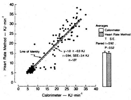
FIG 5. Regression analysis of energy expenditure obtained by the heart-rate method during all possible periods of exercise or rest of the 22 subjects during 22 h in the calorimeter.
