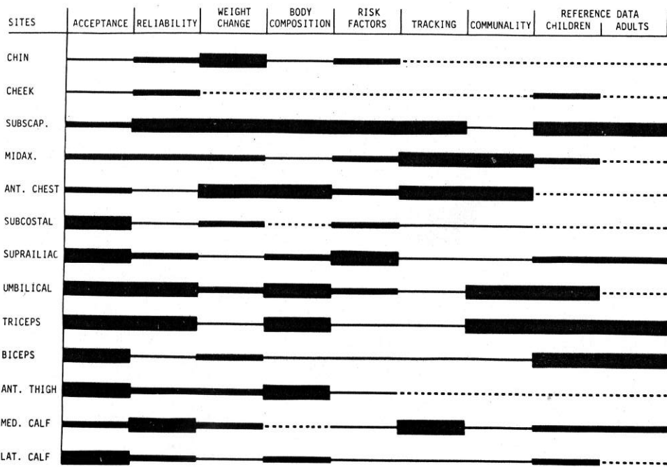
FIGURE 1. A diagrammatic representation of selected skinfold sites graded as good (■), fair (▬), and poor (—) in regard to different criteria. Missing data are represented by an interrupted line (----). Reproduced with permission of Ross Laboratories, Columbus, Ohio, 43216 from Sixth Ross Conference on Body-Composition Assessments in Youth and Adults. p. 16, 1985.
