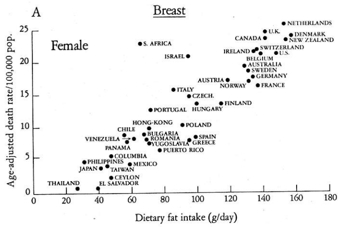
FIGURE 1 Positive correlations between the amount of fat available for consumption in grams per capita per day and age-adjusted mortality from cancers of the breast (A) and colon (B). Reproduced from Carroll and Khor [14] with permission of the publisher (S. Karger AG, Basel).
