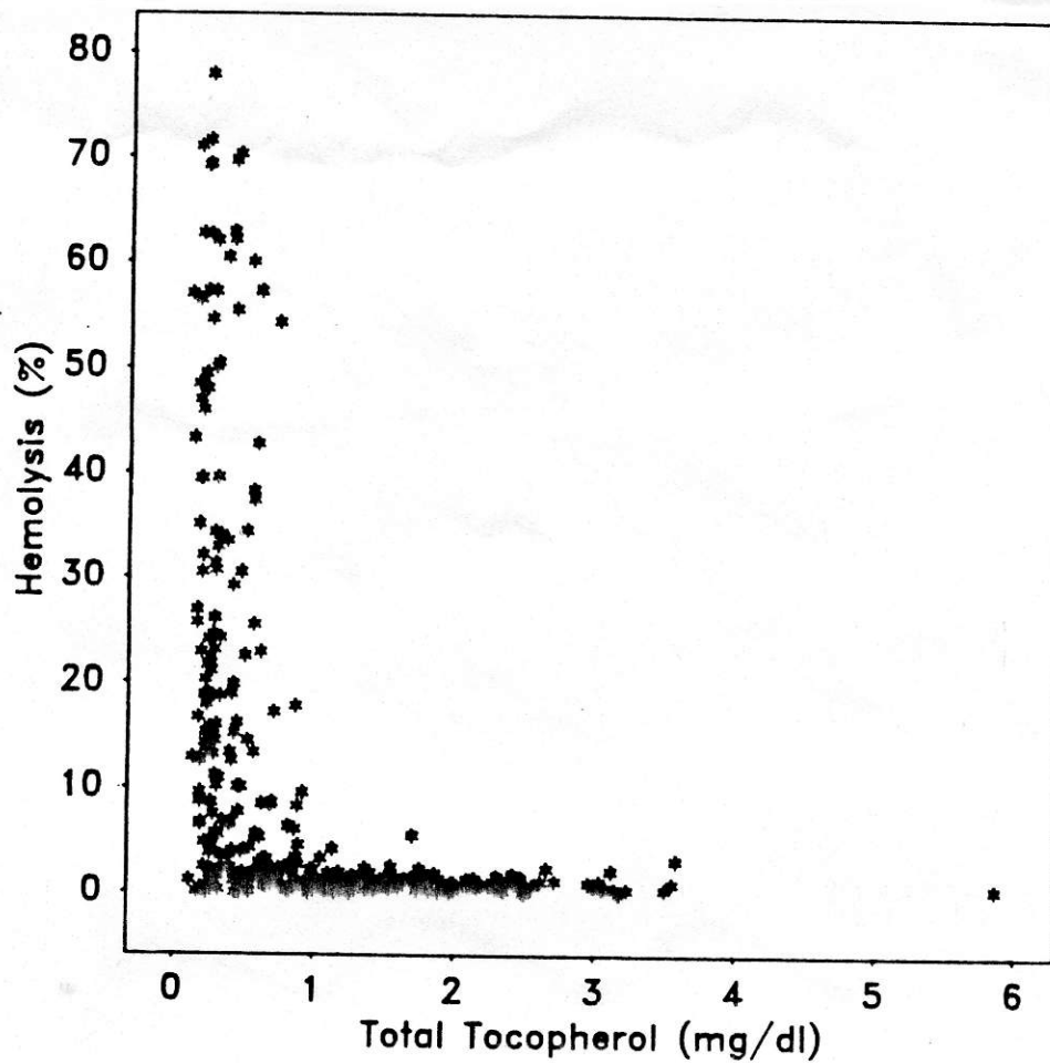
FIG 3. The relationship between the degree of peroxide-induced hemolysis and the plasma TT for all patients
