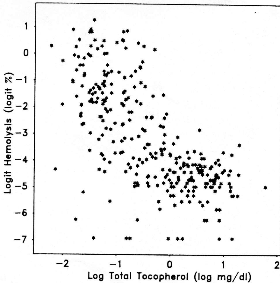
FIG 4. The relationship between the degree of peroxide-induced hemolysis and the plasma TT for all patients and all days. Data transformed as logit %H = logarithm [%H/(100-%H)] and logarithm TT.
